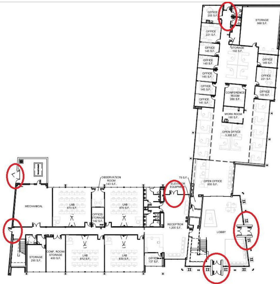
A FIRST FLOOR
